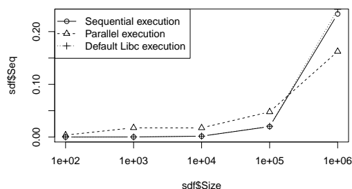
Figure 1. Comparing performances of several implementation of the quicksort algorithm
